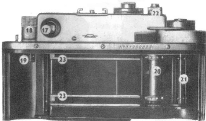
Fig. 3. Rear view of camera with cover removed. 17—range-viewfinder eyepiece; 18—film rewind knob; 19—cassette spool guide; 20—sprocket; 21—take-up spool; 22—shutter disengaging bush; 23—film track slide
